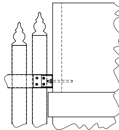
DETAIL G SCALE 1 : 10
