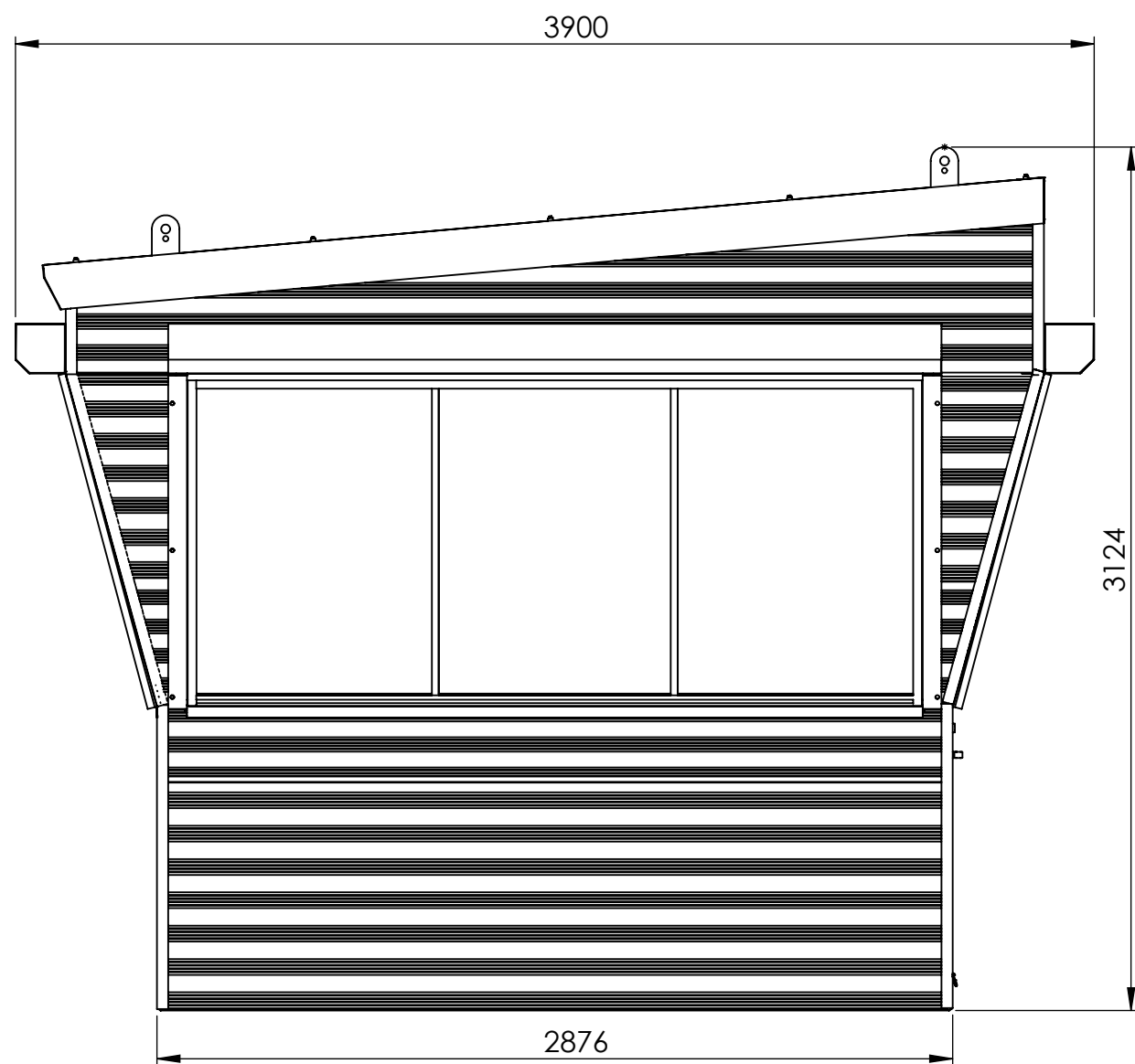
TUMORRAMA FIRE CABIN - 3 x SPRING LOADED SHUTTERS & A/C WEIGHT - 1851 kg
