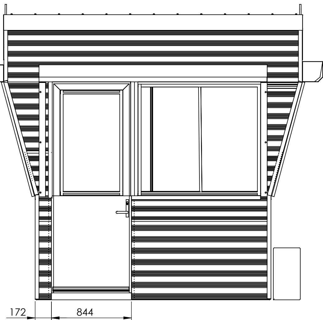
TUMORRAMA FIRE CABIN - 3 x SPRING LOADED SHUTTERS & A/C WEIGHT - 1851 kg
